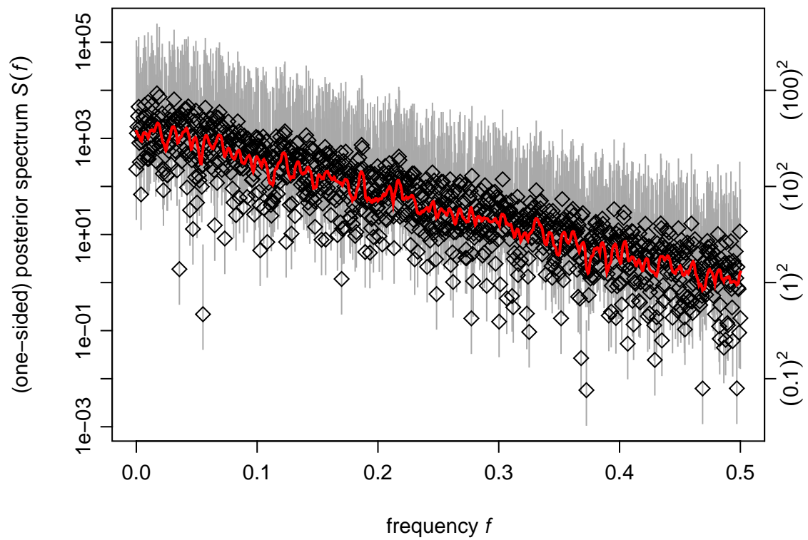
Figure 6: Project MAGNET PSD estimates from bsspec , a Bayesian method, compared to the psdcore results shown in Figure 4.
